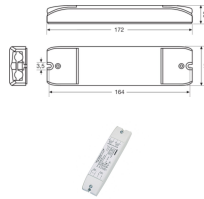
Technische Daten Osram LED driver Optotronica CV 1-10V | Dimmbar
